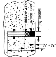
DETAIL "A" USE THIS DETAIL IN CONNECTION WITH TYPE TCU (SECTION A-2) AND TYPE L-J JOINT (SECTION D-1) AND NOTES (C) THROUGH (F).
