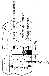
DETAIL "B"
